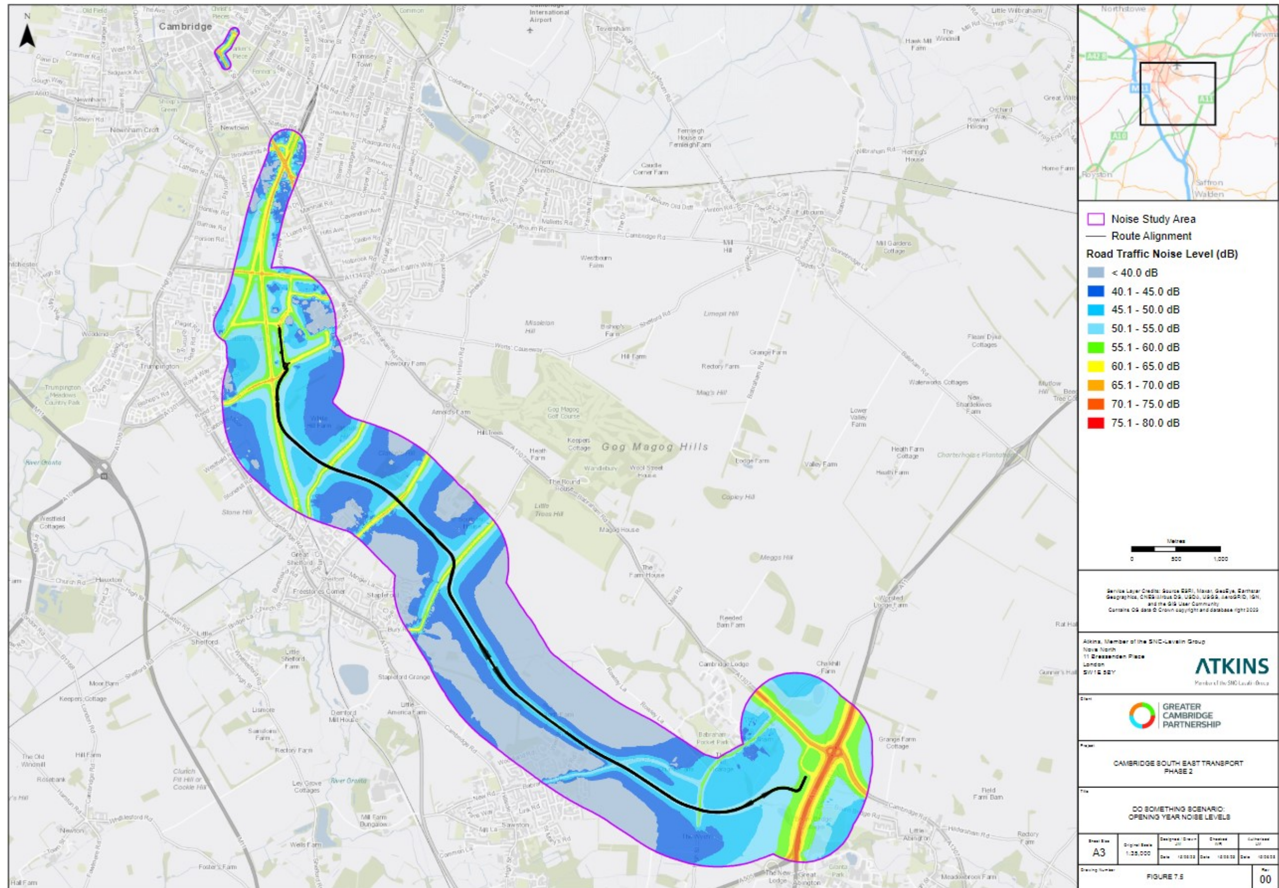
Figure 7.5.3 Do something opening year noise levels
