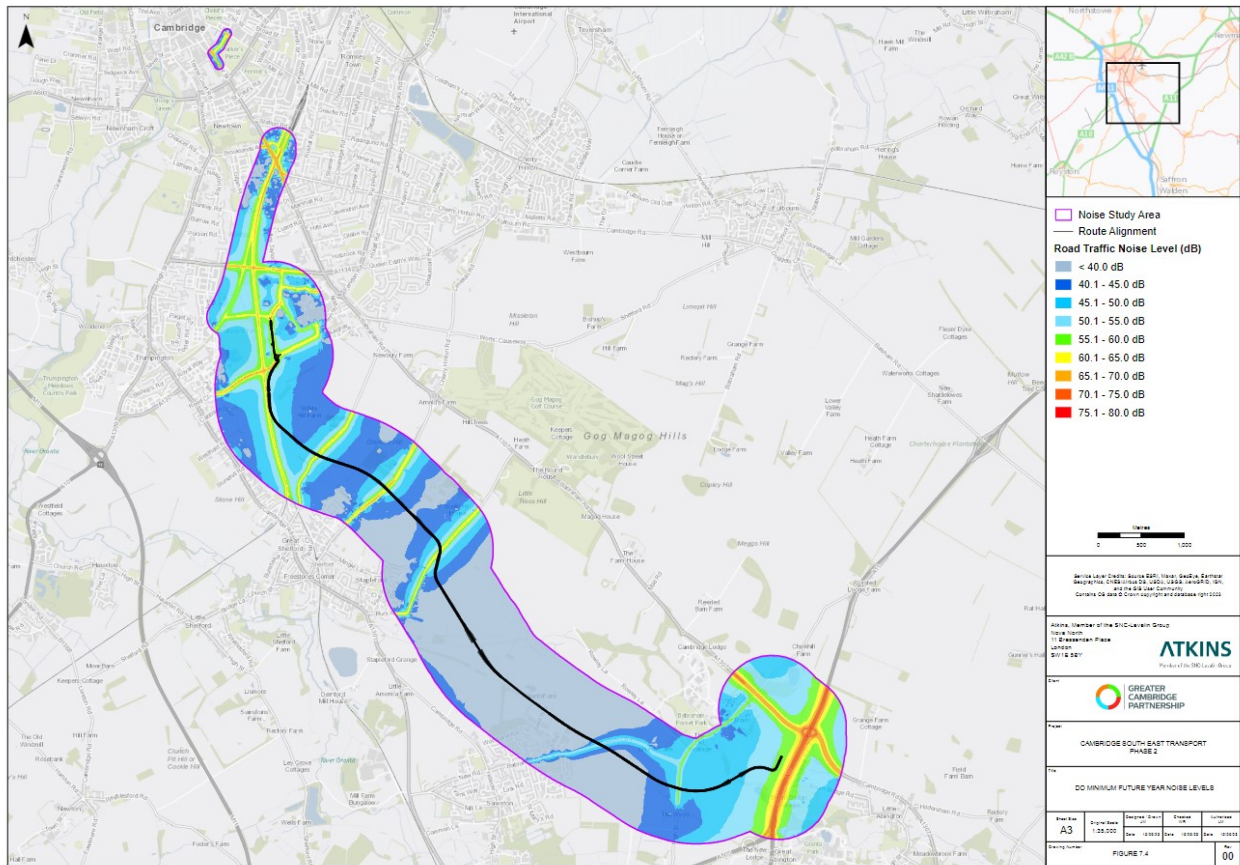
Figure 7.5.2 Do minimum future year noise levels
