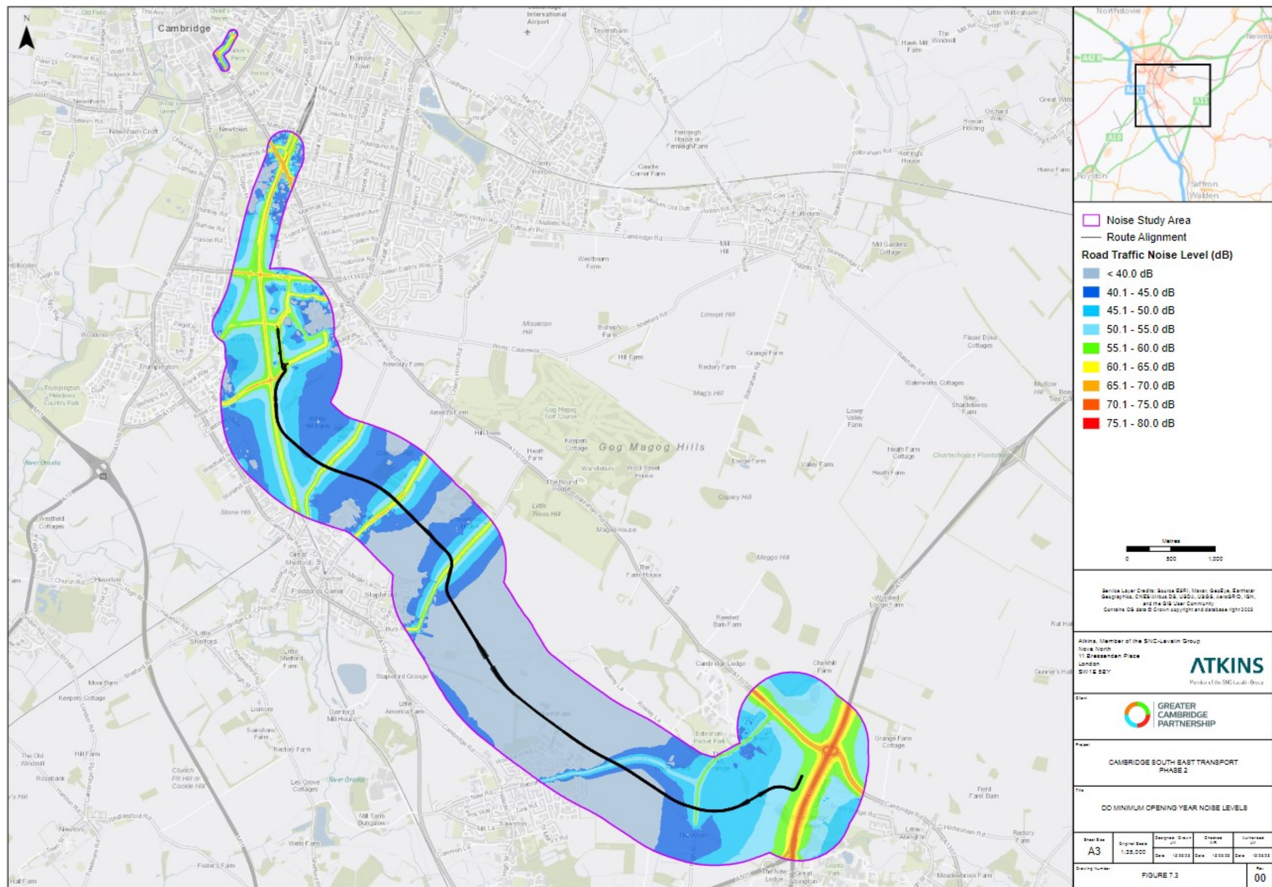
Figure 7.5.1 Do minimum opening year noise levels
