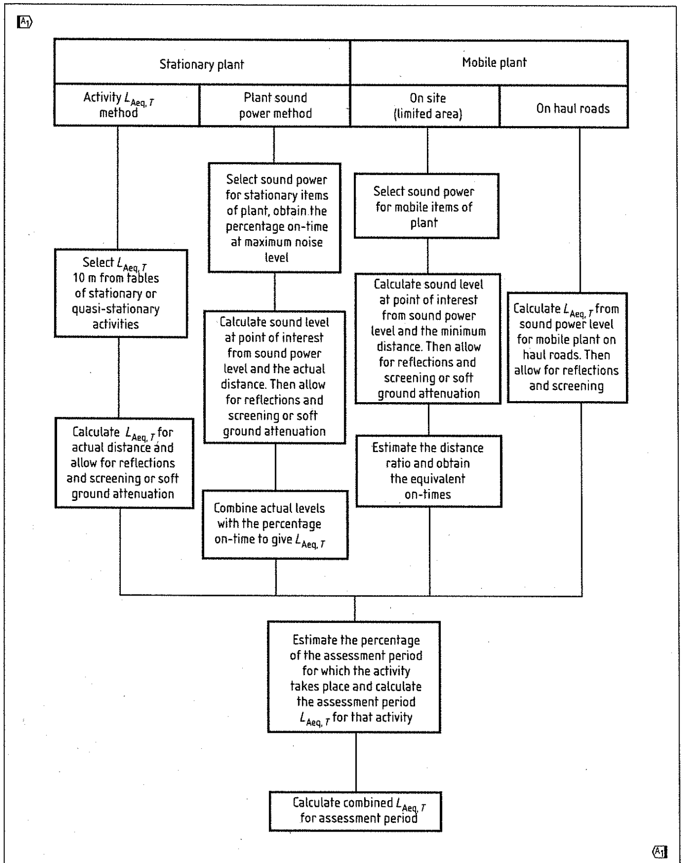
Figure E.1 Flow chart for the prediction of site noise
