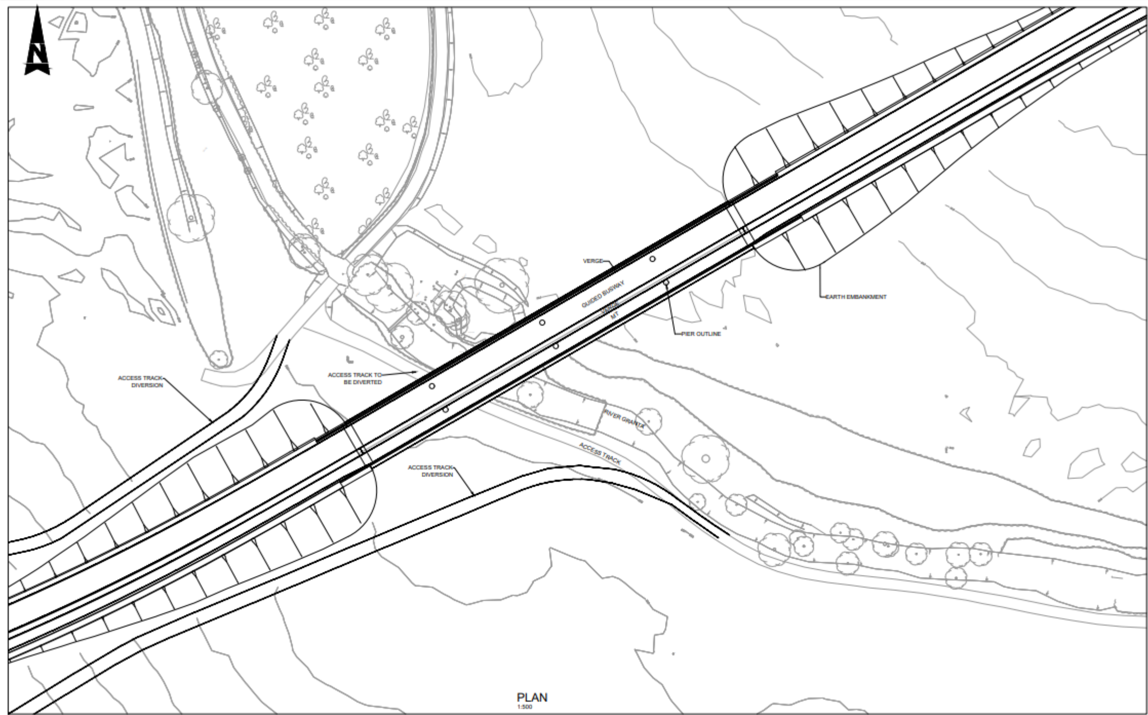
Figure 47: Section from engineering drawings – Structure 8 Babraham Viaduct
