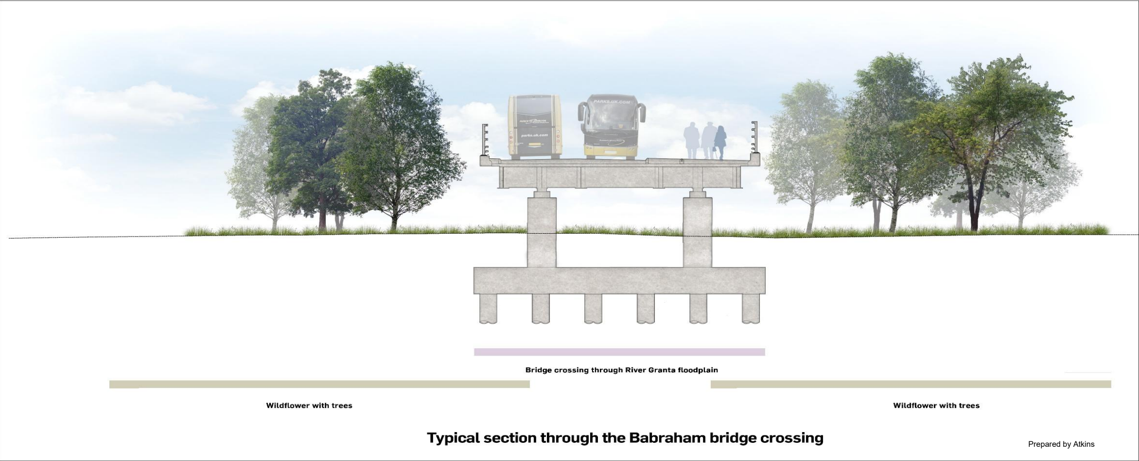
Figure 48: Section showing the Babraham bridge crossing in the context of the landscape design (planting shown at year 15)
