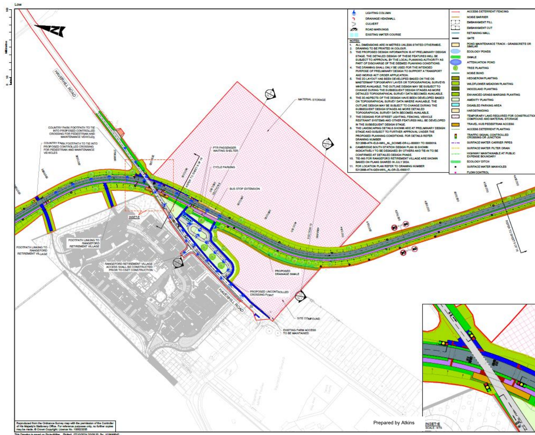
Figure 21: Stapleford stop and Haverhill Road crossing plan (Deemed Planning Drawings Sheet 7 of 16)
