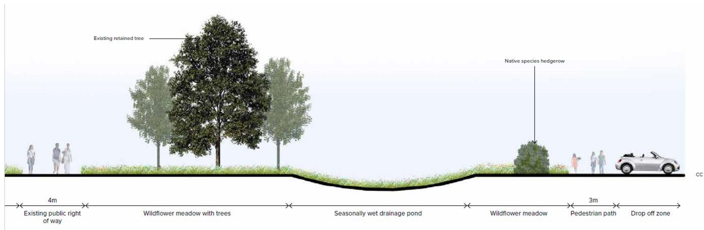
Figure 64: Section showing the relationship between the drop off zone, swale and existing PROW in central car park
