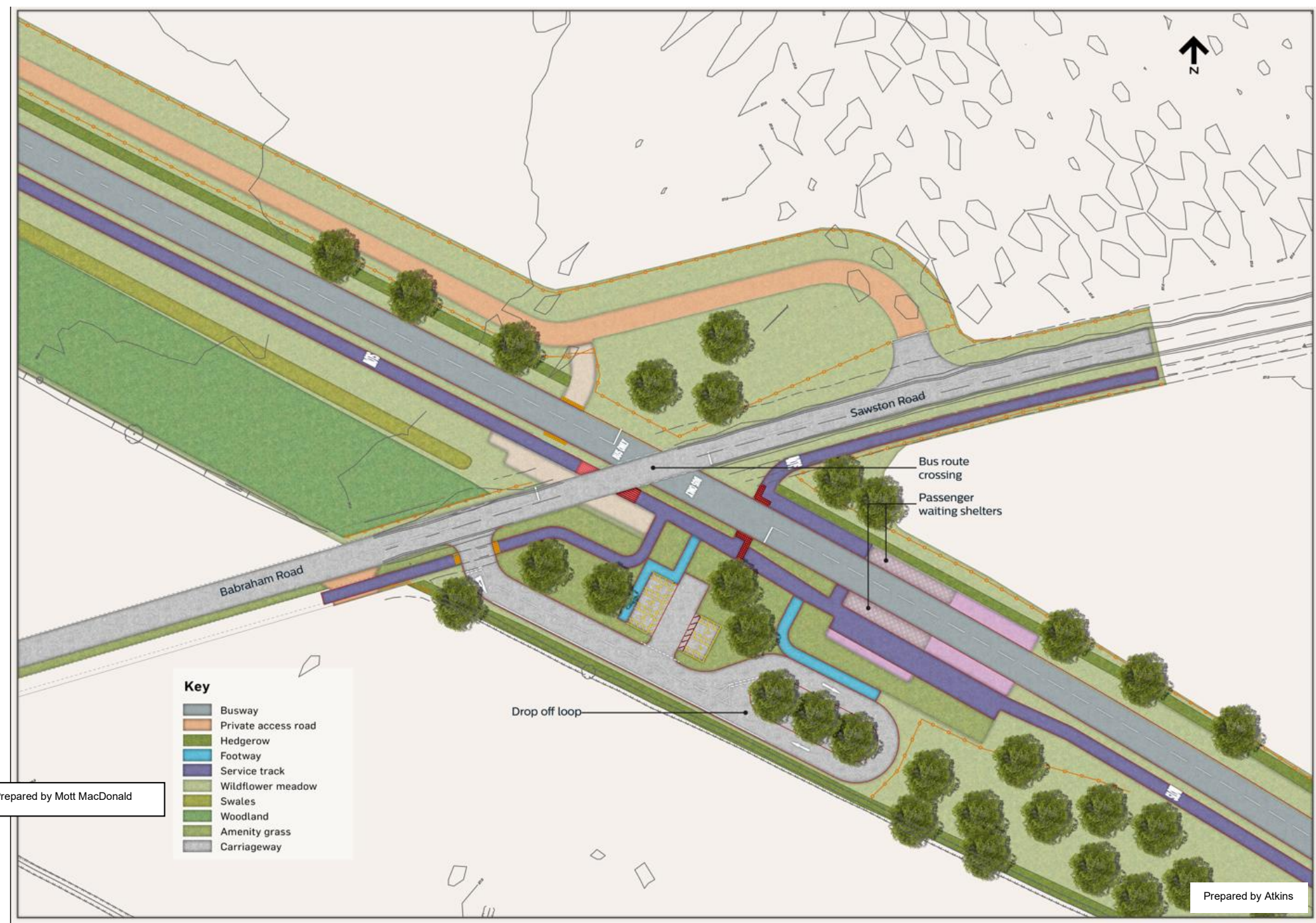
Figure 38: Busway route and junction layout plan
