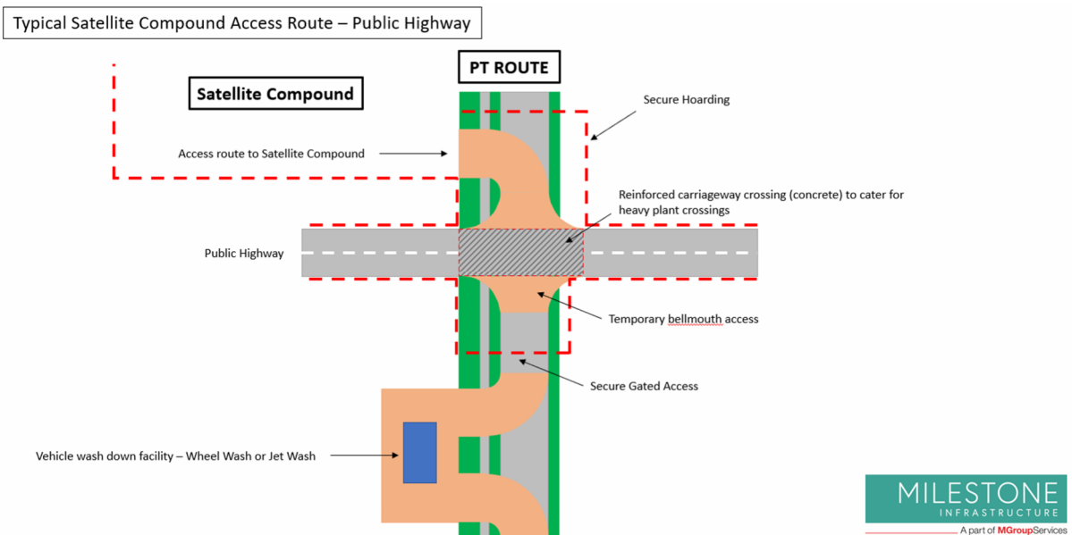
Figure 7: Typical satellite compound access route – public highway
