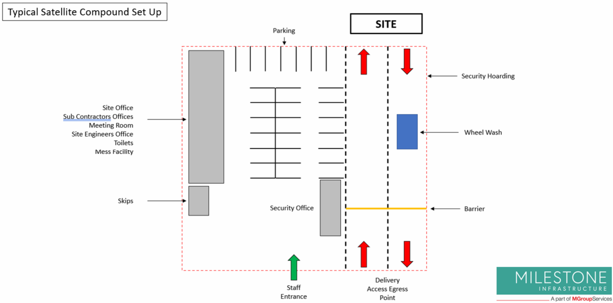
Figure 6: Typical satellite compound set up
