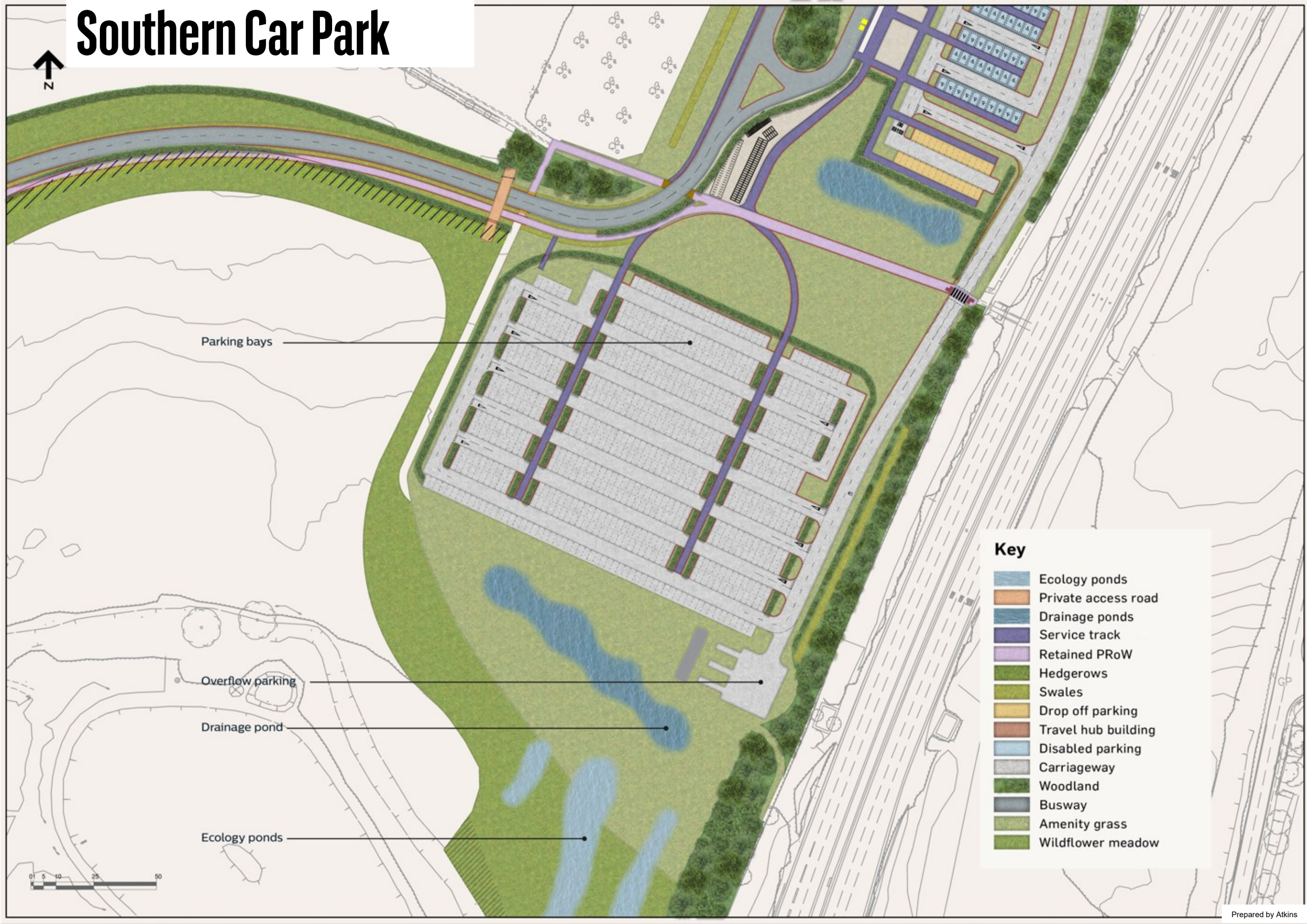
Figure 58: Southern Car Park
