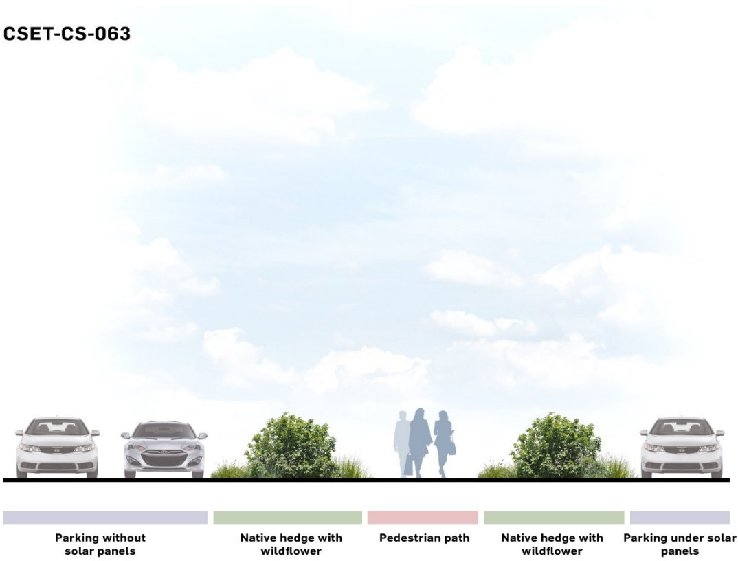
Typical section showing planting and pedestrian route through parking area
