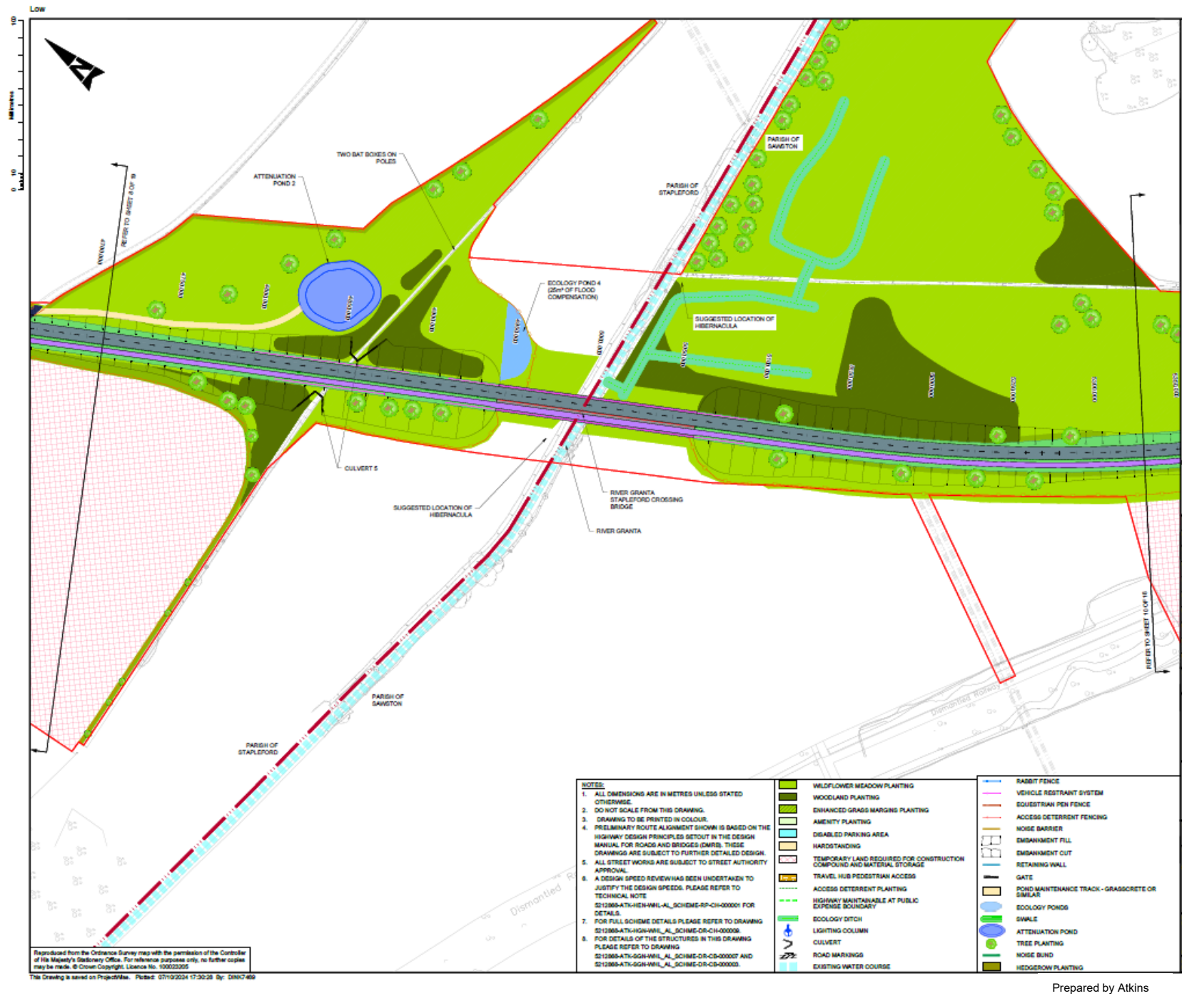
Figure 29: Busway route and landscape plan (Landscape Layout Sheet 9 of 18)
