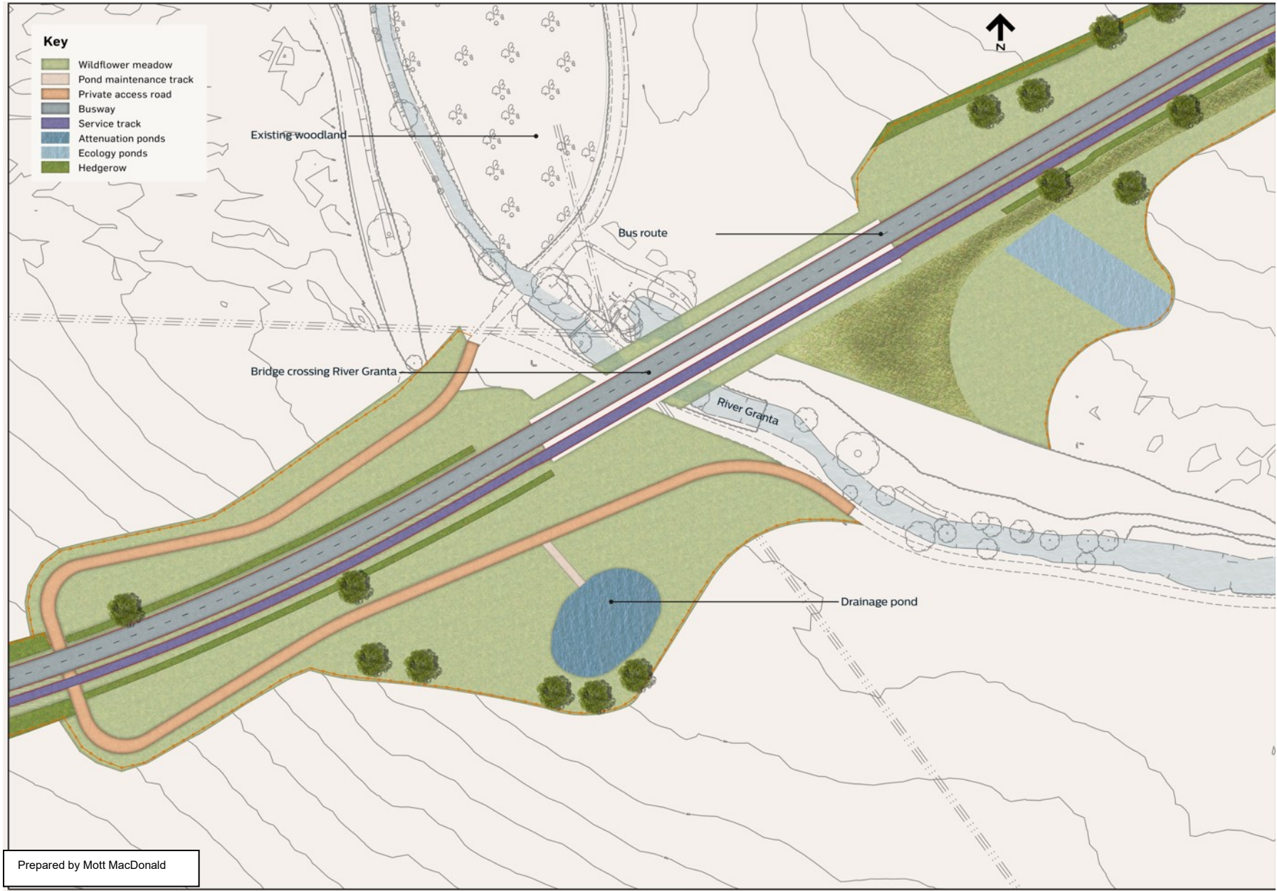
Figure 46: Busway route and layout
