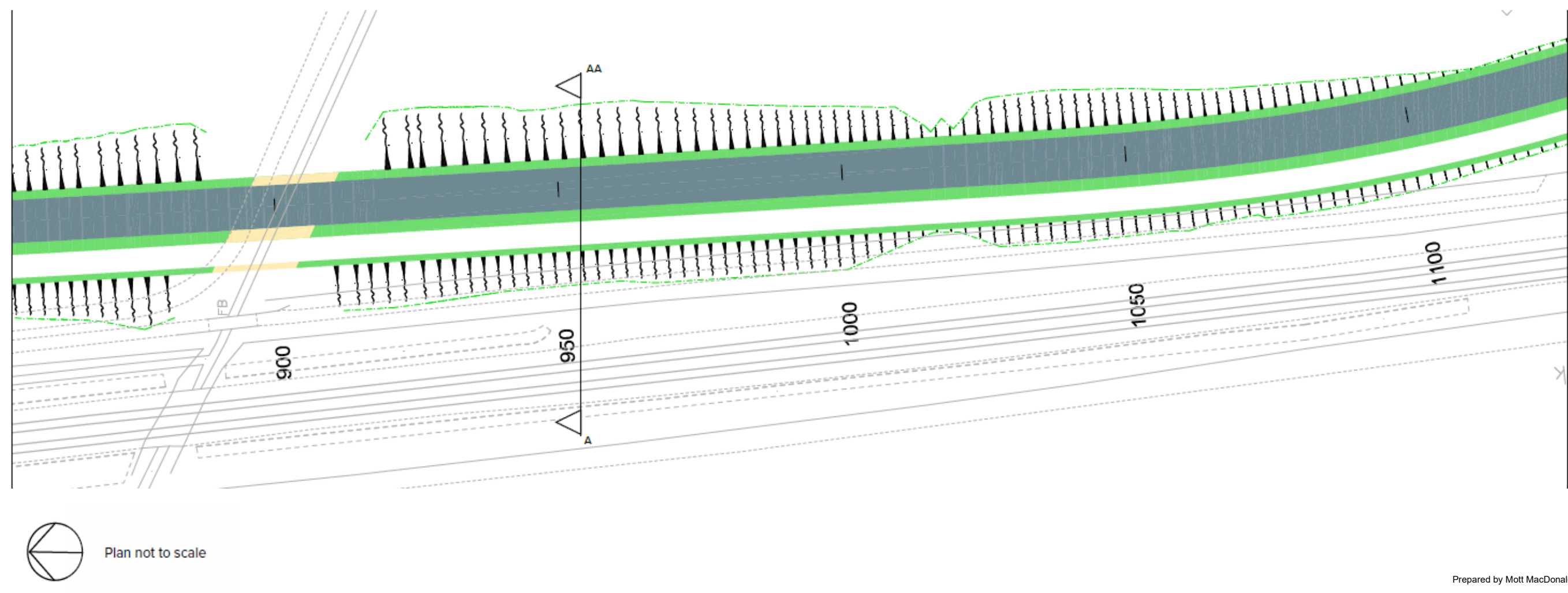
Figure 9: Section from engineering drawings
