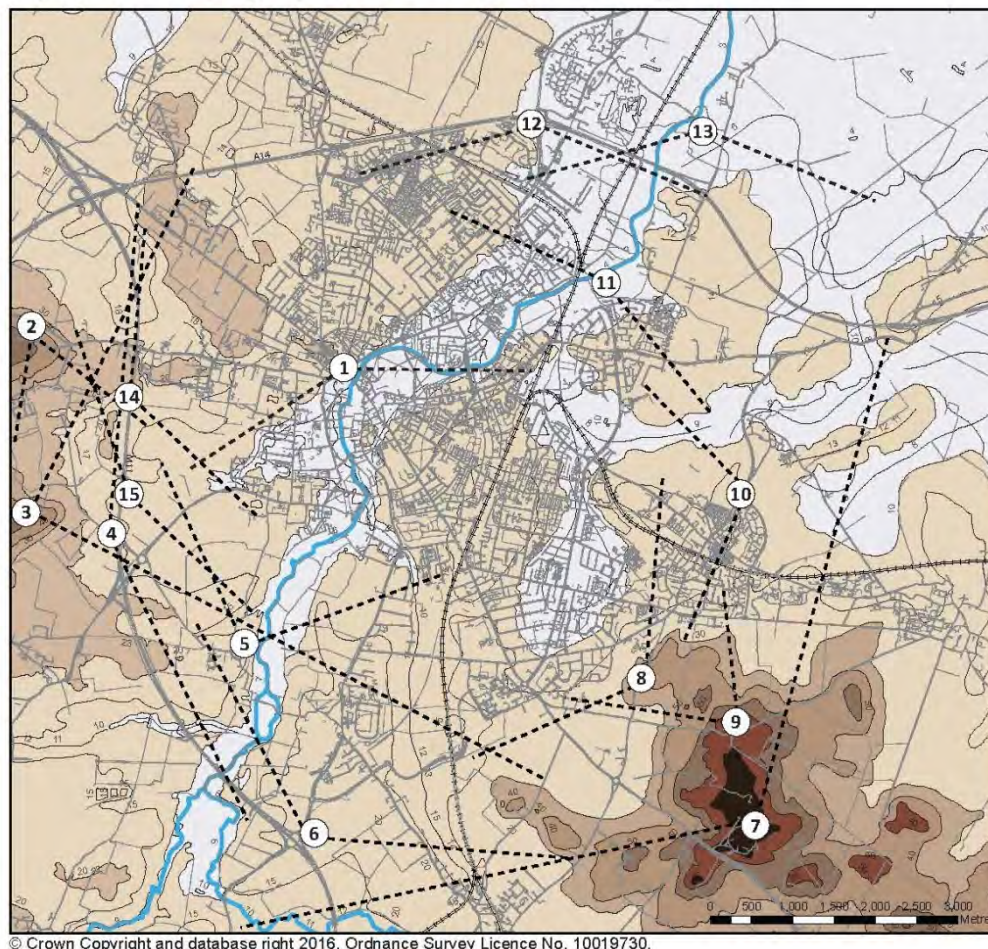
Figure F.3 Topography and Strategic Viewpoints
