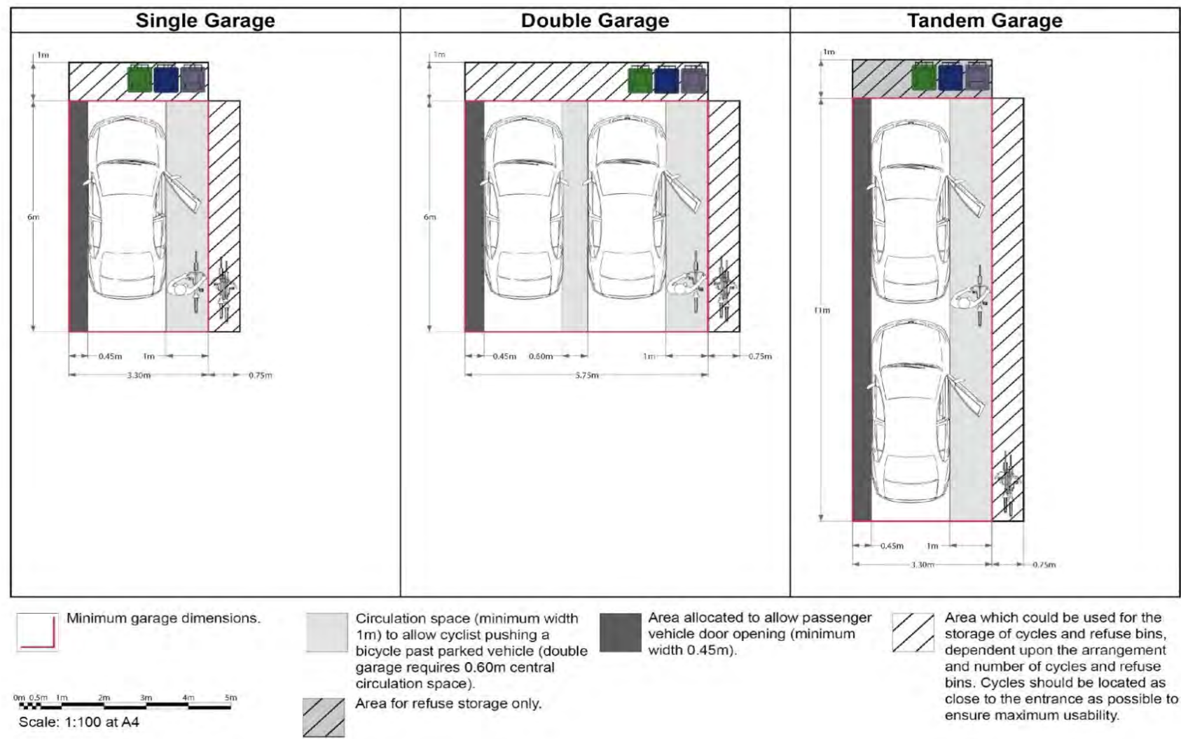
Figure L.1: Garage dimensions
