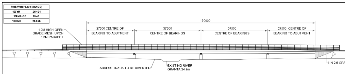
Figure 10 Elevation of the proposed River Granta (Babraham) Crossing Bridge (all dimensions are in mm) [CD1-12-08, page 10]
