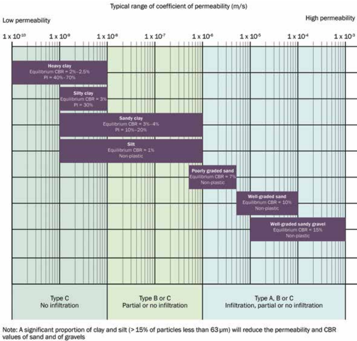
Figure 20.17 Soil classification guide (after Interpave, 2010)
