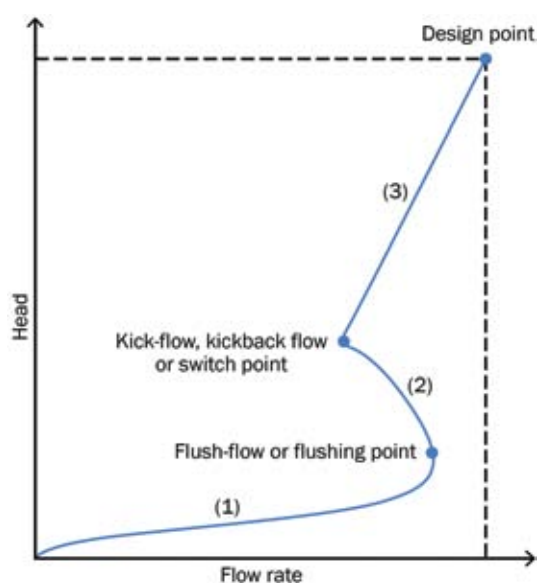
Figure 28.21 Example of head–discharge relationship for passive devices (vortex flow controls) (courtesy Hydro International)
