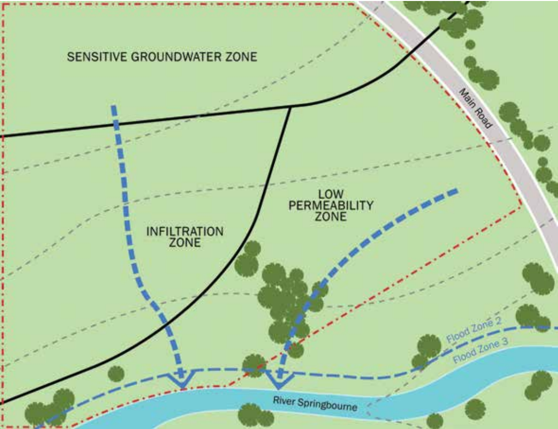
Figure C.1 Site characterisation
