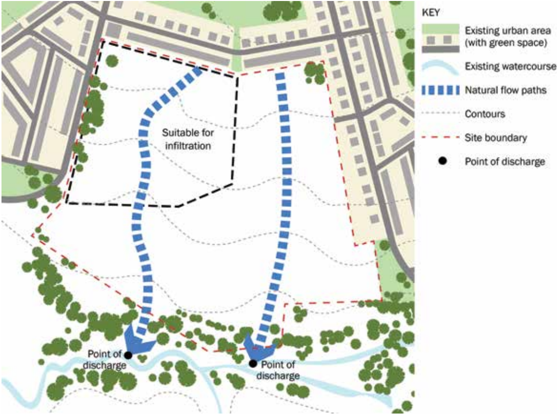
Figure 7.4 Characterising flow routes and discharge points
