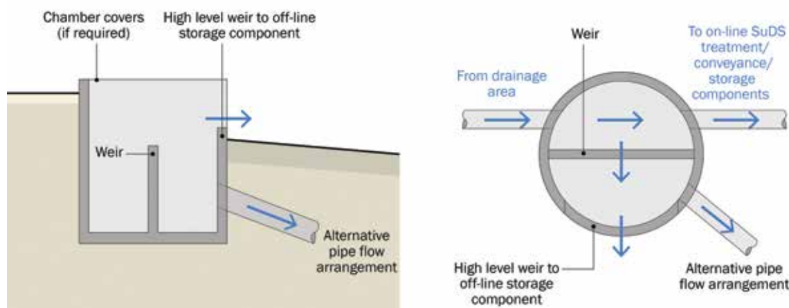
Figure 28.12 Conceptual design for engineered inlet flow divider
