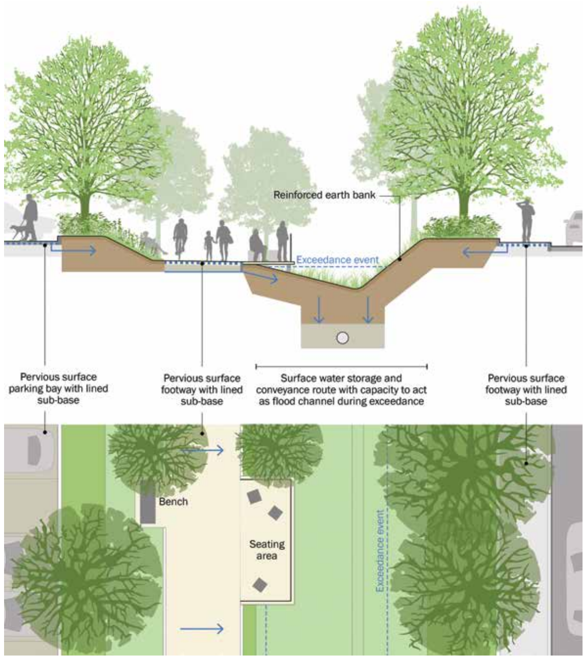
Figure 10.28 Typology 9 – Greenway
