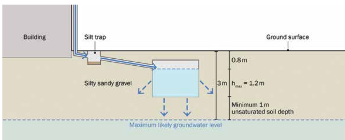
Figure C.6 Residential soakaway
