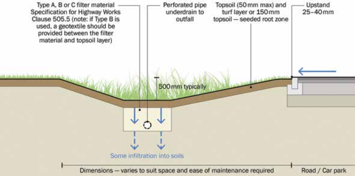
Figure 9.15 Swale detail
