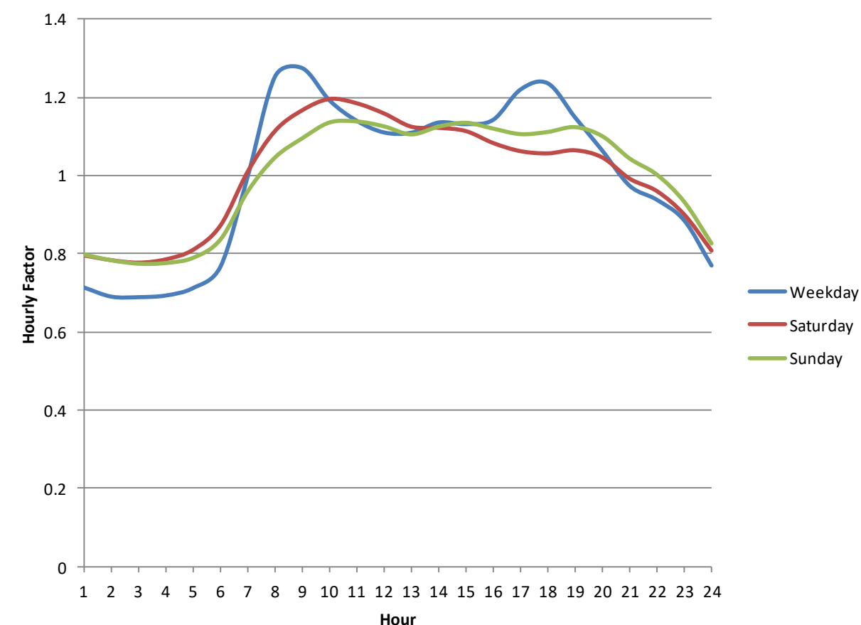
Figure A6.1.2 Diurnal profiles for grid sources
