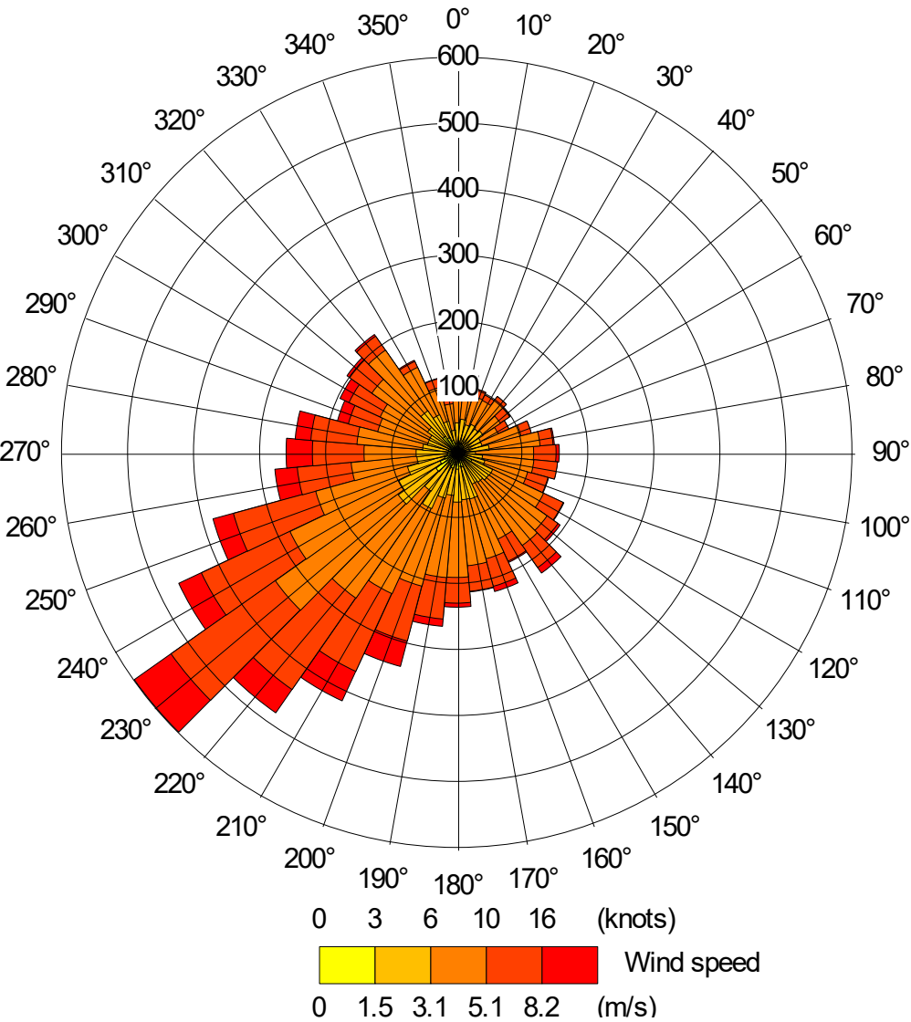
Figure A6.1.3 Wind rose for Mildenhall, 2019
