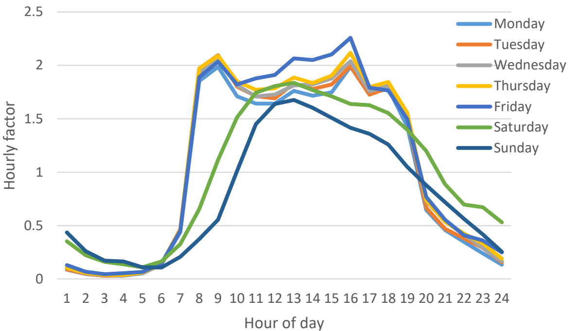
Figure A6.1.1 Diurnal profiles for Cambridge
