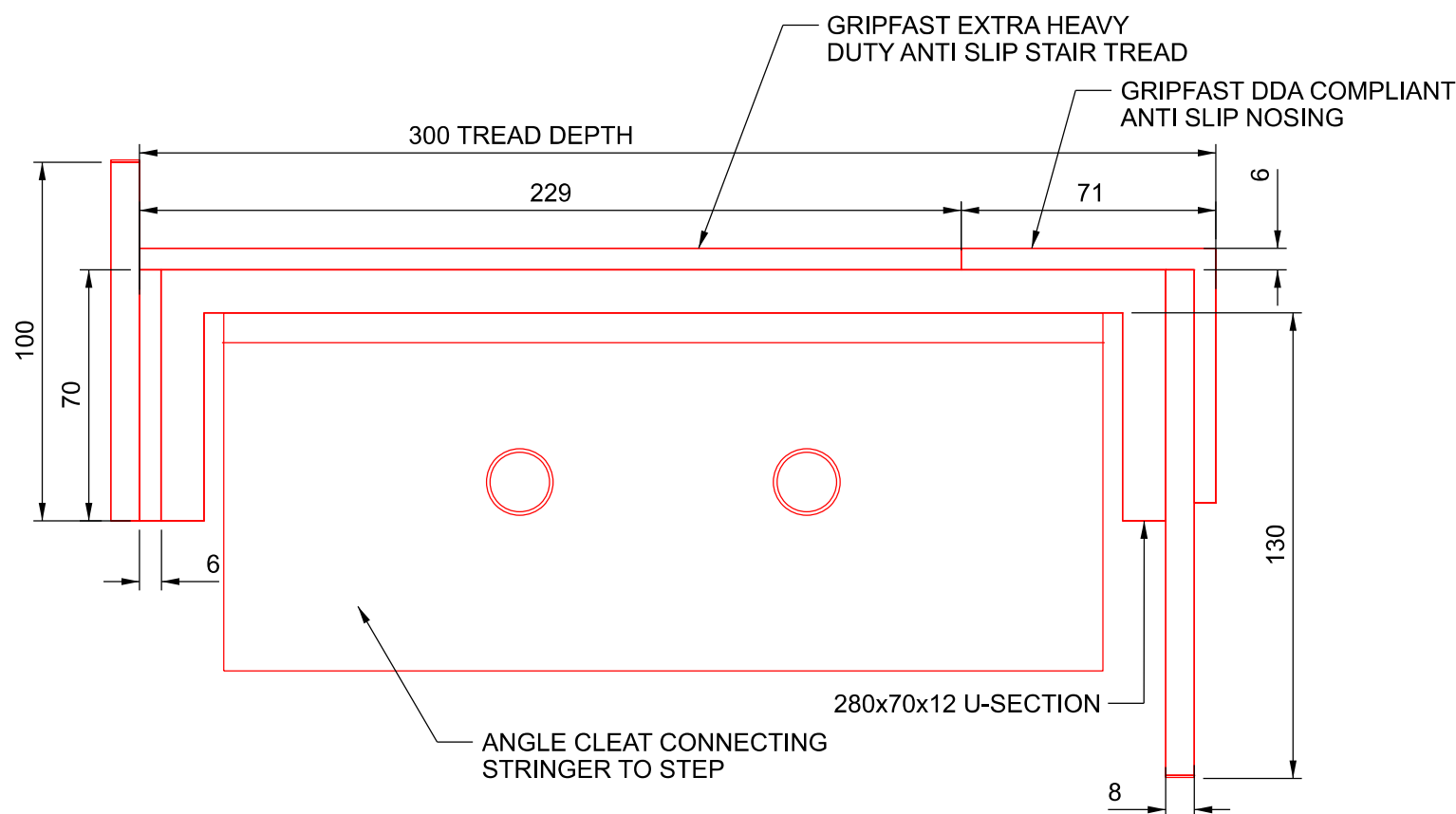
CROSS SECTION SHOWING STEP COMPONENTS
