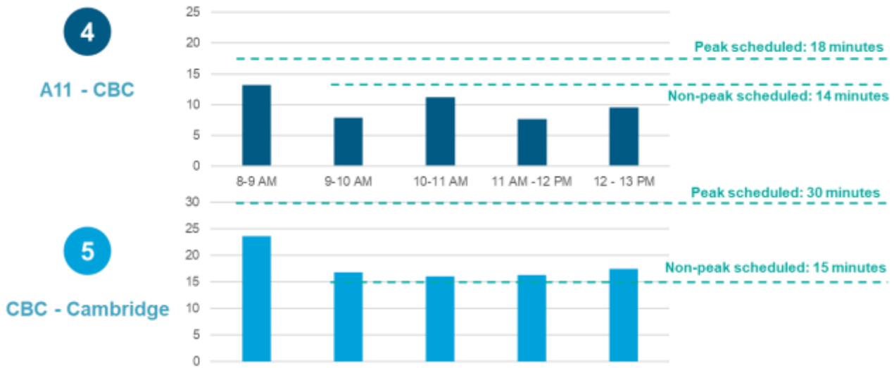
Figure 1-28 - Route 13 – journey time by hours (selected sections only)
