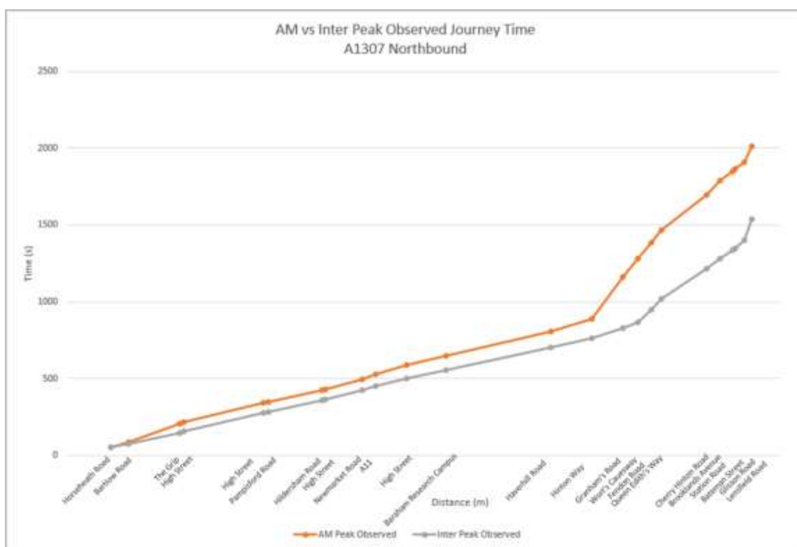
Figure 1-20 - Northbound journey time along the A1307 in AM peak (weekday 2019) 49
