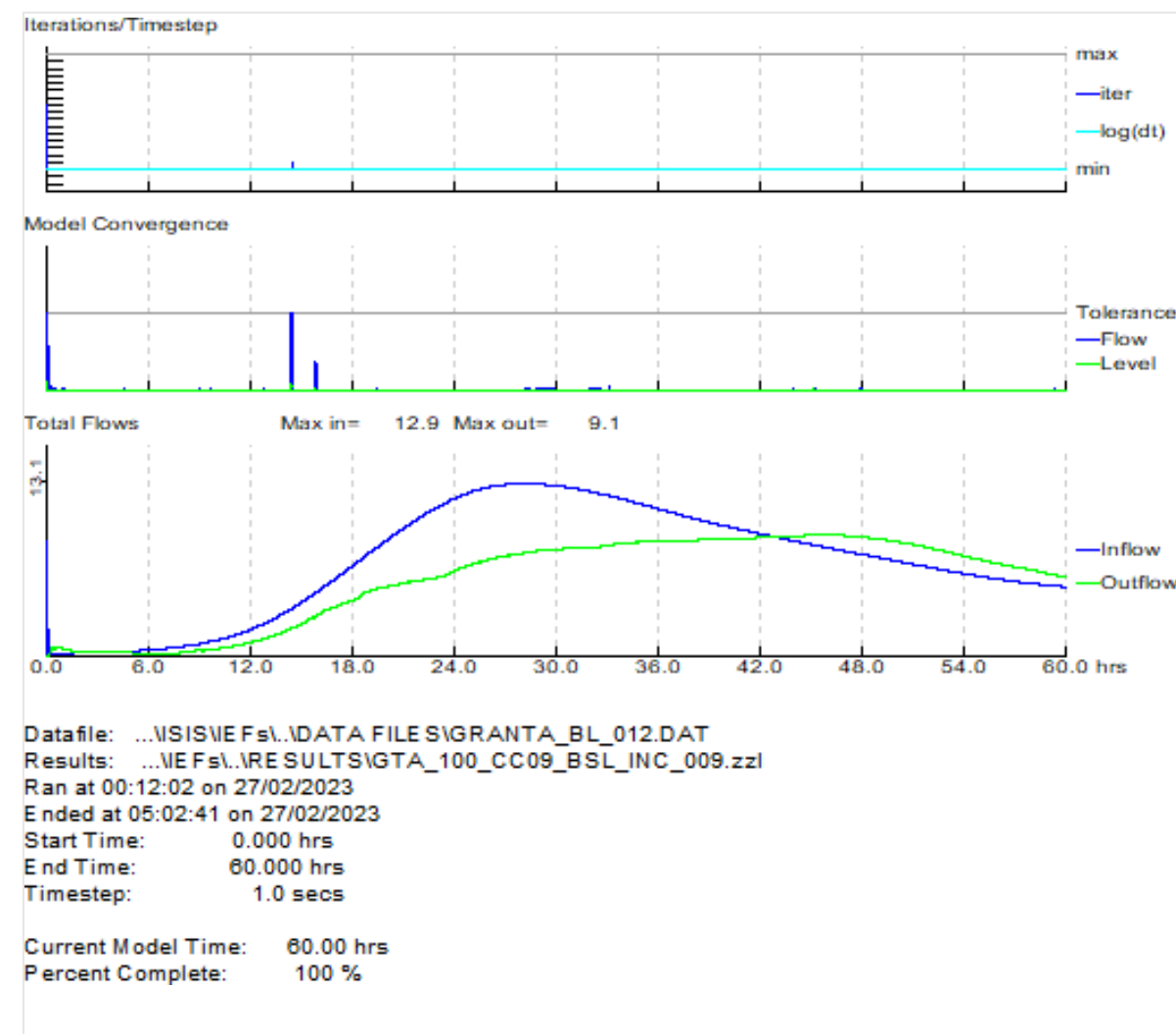
Figure A8.2.4 Flood modeller - Model convergence plot
