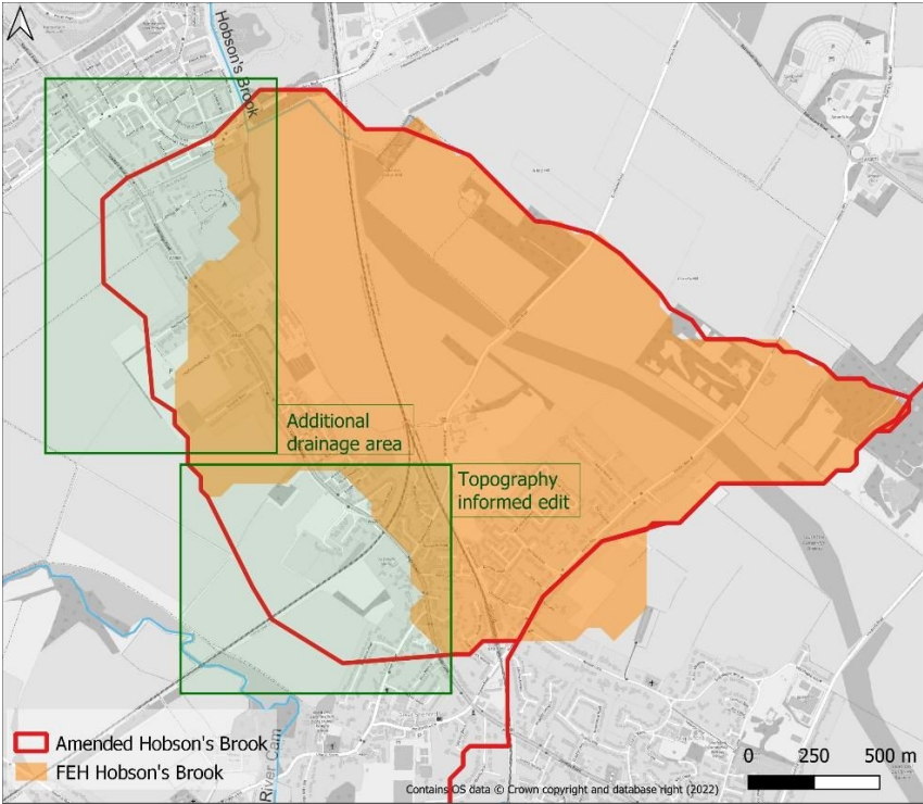
Figure 2 Hobson's Brook catchment area amendment
