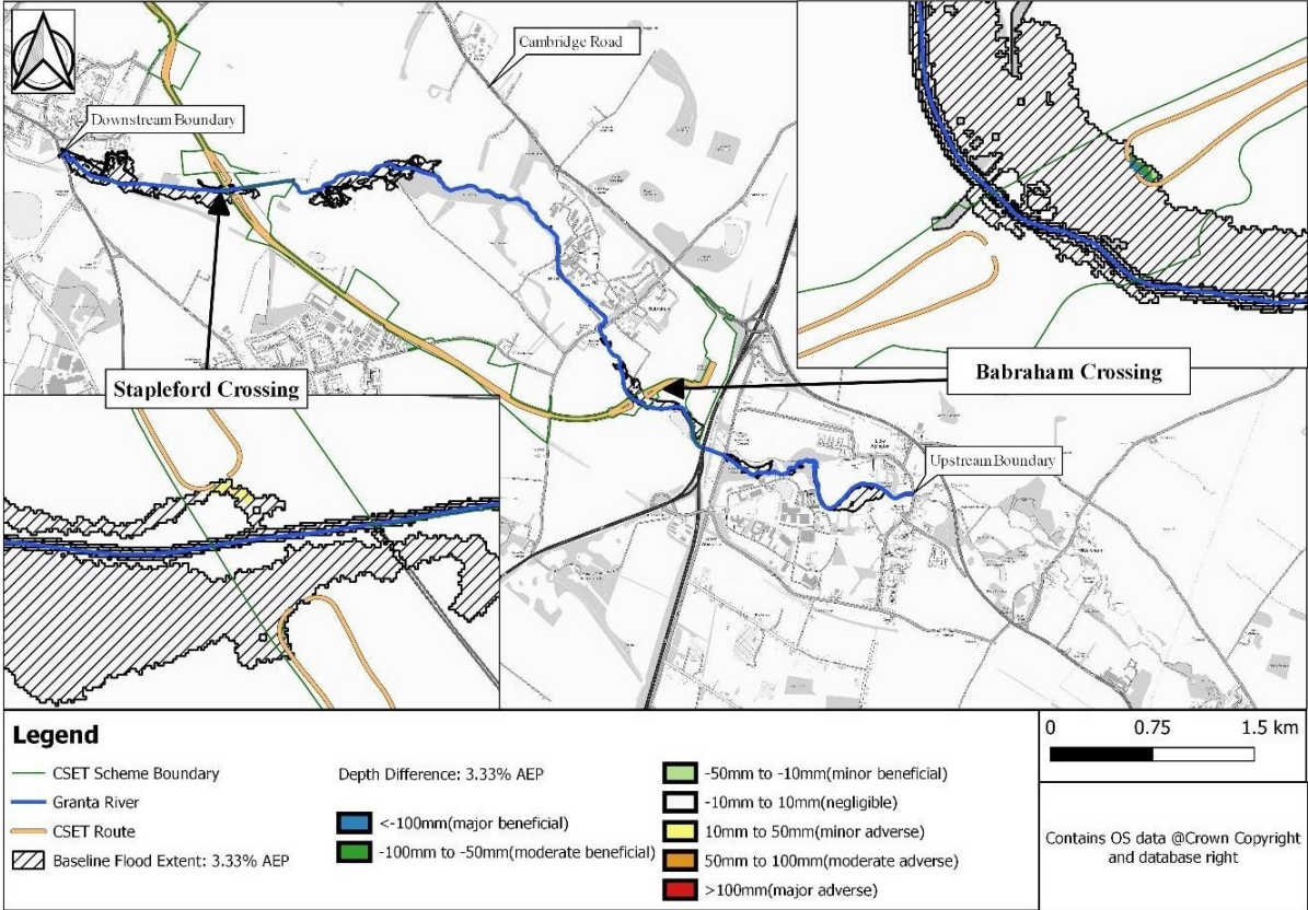
Figure A8.2.9 Depth difference for 3.33% AEP event
