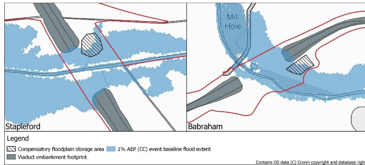
Figure A8.2.19 Floodplain compensation areas
