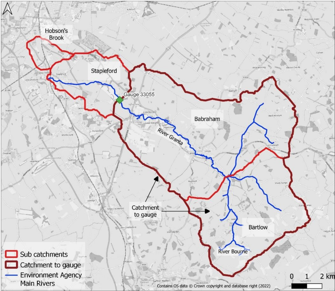
Figure A8.2.1 Subcatchment locations
