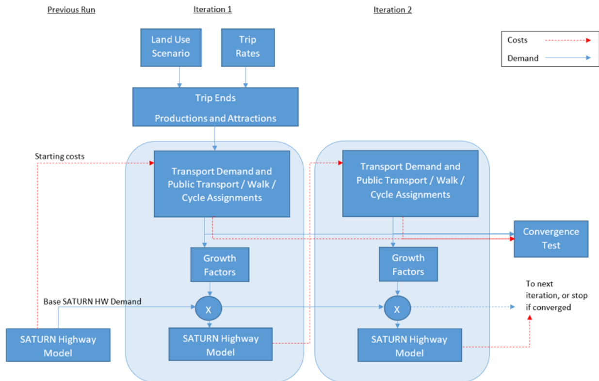
Figure 1-1 Model Structure Schematic
