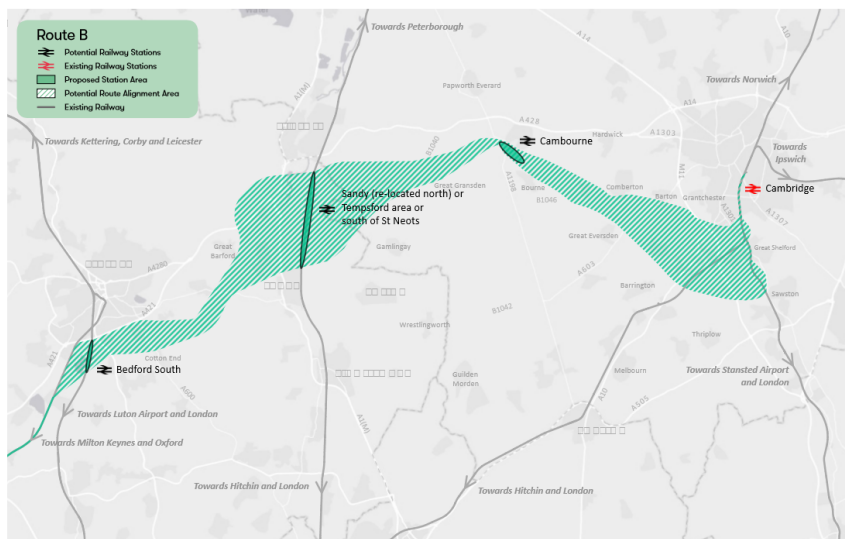
Figure 27: East West Rail Central Section – Cambourne Options
