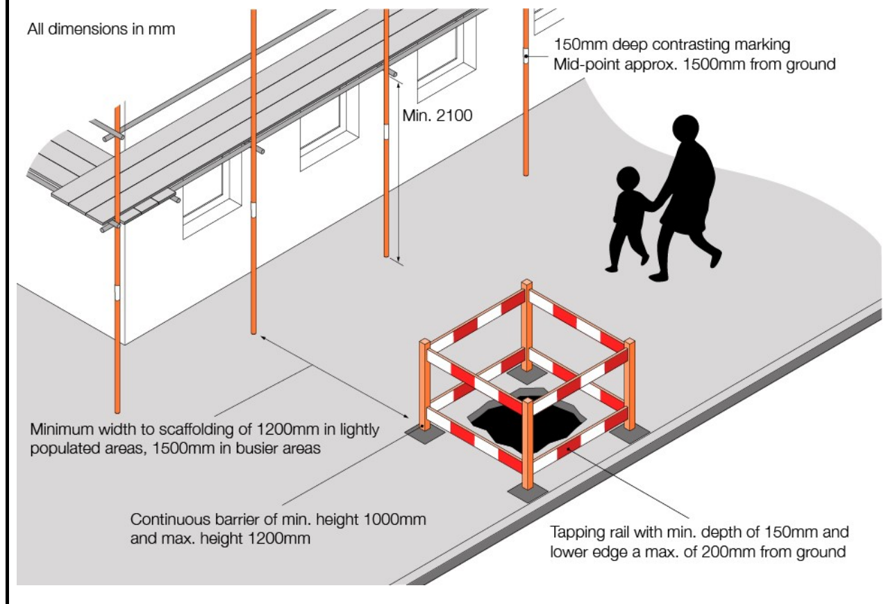
Figure 3: Street works protection
