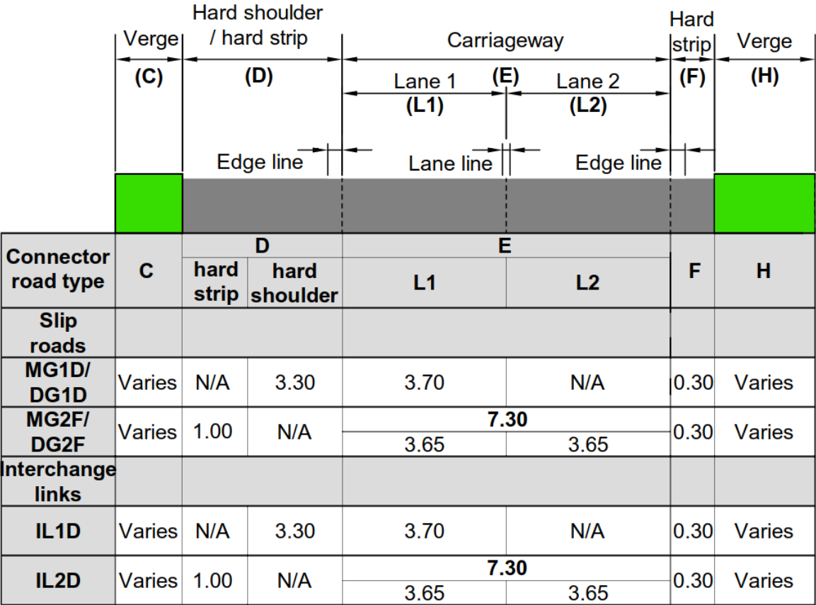
Figure 2.1.1N1h Dimensions of cross-section components for urban all-purpose connector roads
