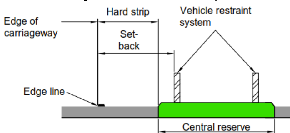
Figure 2.25c Offside - with hard strip
