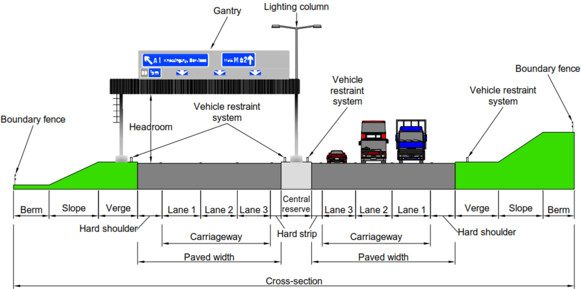
Typical rural motorway cross-section components
