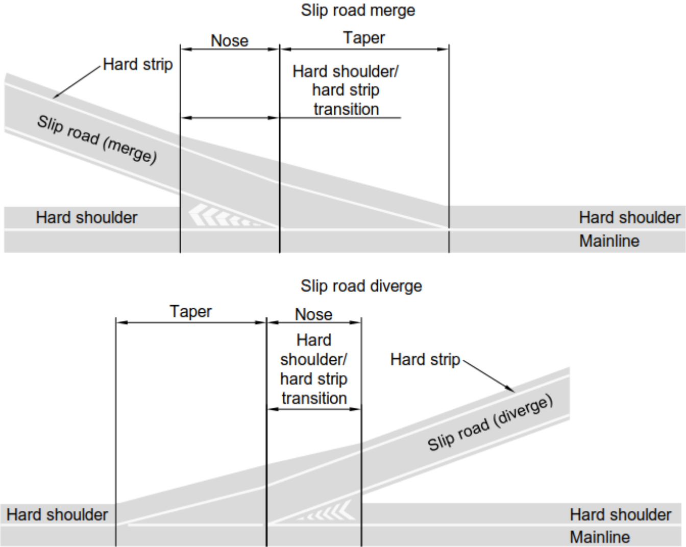
Figure 2.30a Hard shoulder / hard strip transitions for motorways
