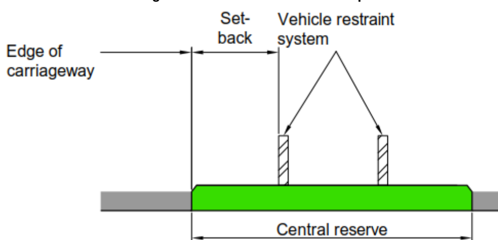
Figure 2.25d Offside - no hard strip
