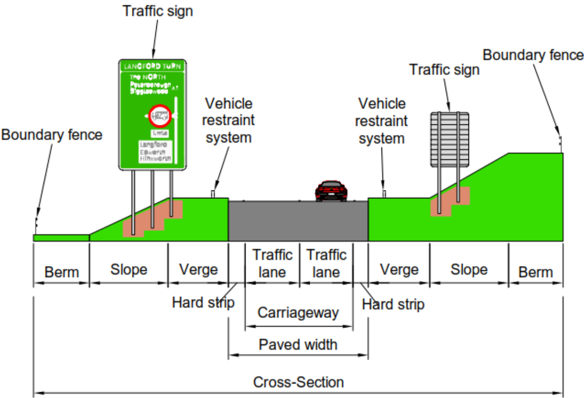
Typical rural single carriageway cross-section components
