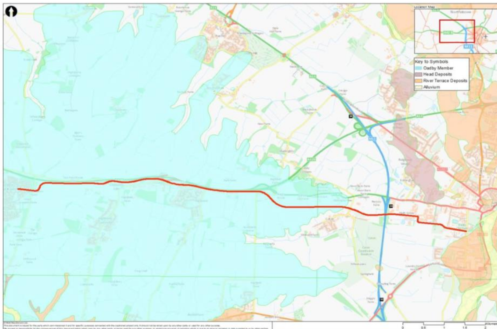
Figure 5-9 – Superficial geology
