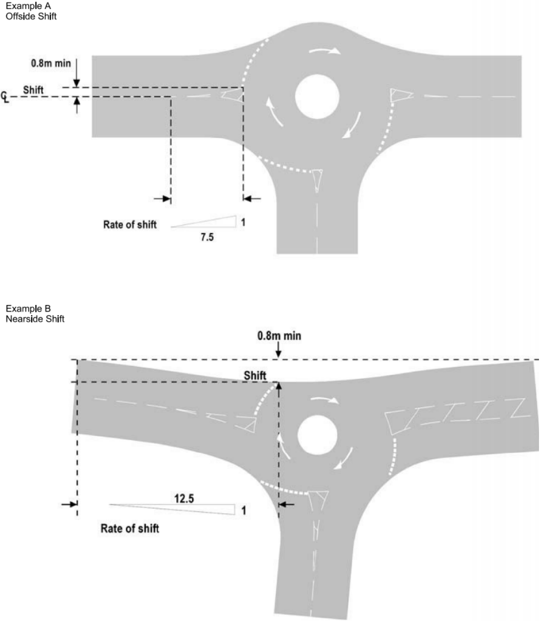
Figure 5.18.3 Illustration of lateral shift
