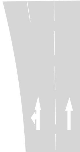
Figure 3.27.6b Example of entry markings
