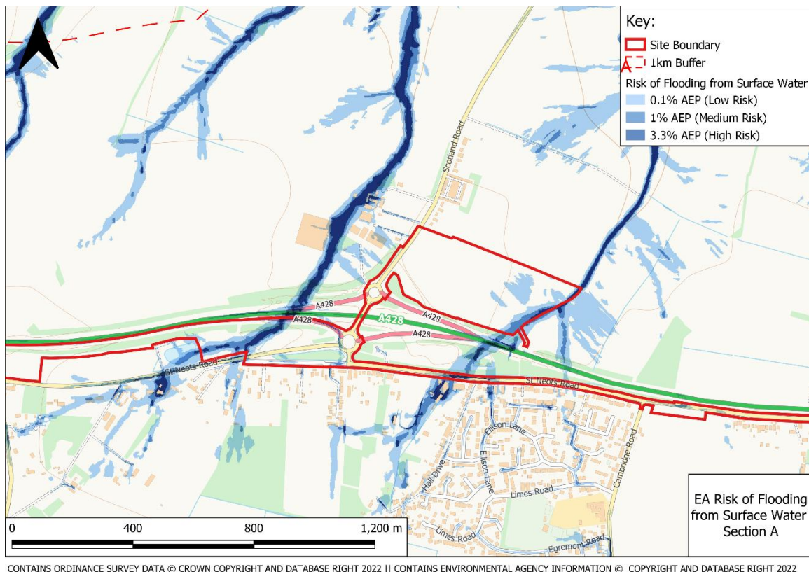
Plate TR13.1-4-8 – Section A surface water flood risk
