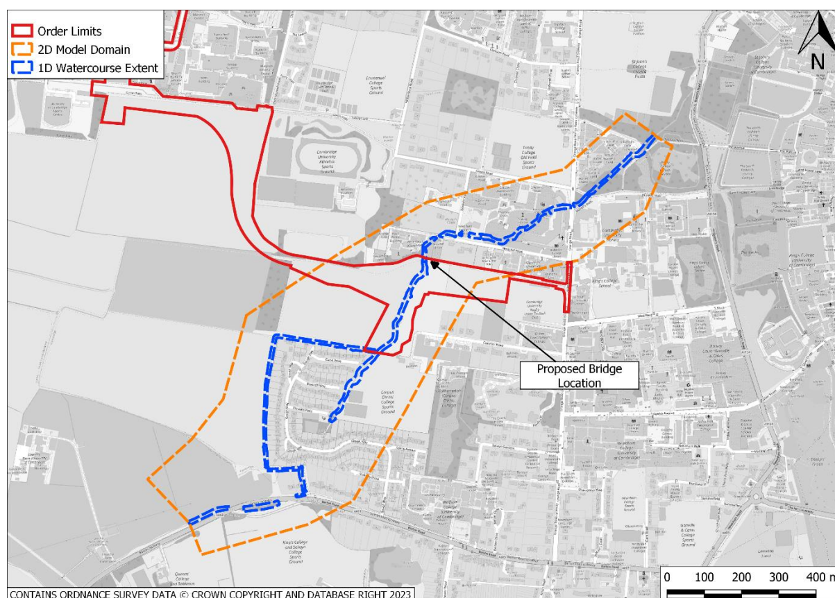
Plate TR13.1-1-1 – Hydraulic model extents
