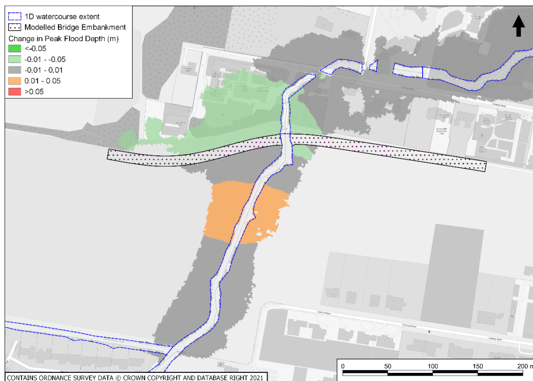
Plate TR13.1-1-3 – Baseline vs Proposed (10m span with existing footbridge removed) change in peak flood water level for the 1% AEP with 19% climate change allowance
