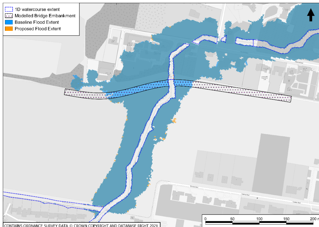
Plate TR13.1-1-2 – Baseline vs Proposed (10m span with existing footbridge removed) flood extent for the 1% AEP with 19% climate change allowance
