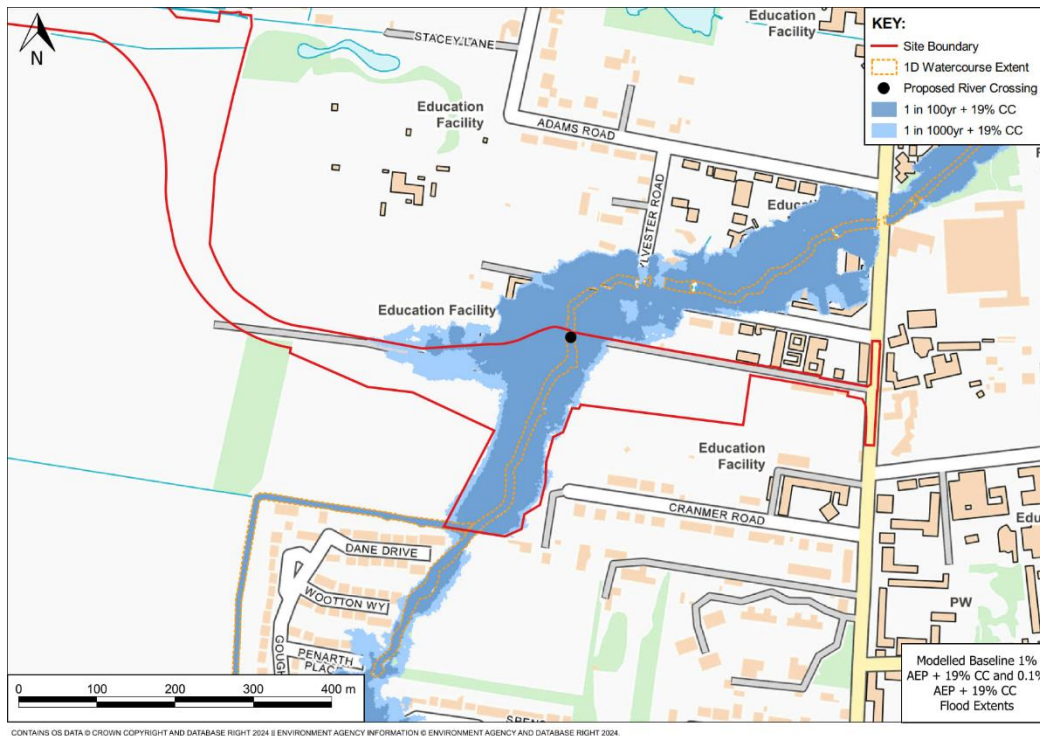
Plate TR13.1-4-5 – Modelled baseline 1% AEP + 19% CC and 0.1% AEP + 19% CC flood extents
