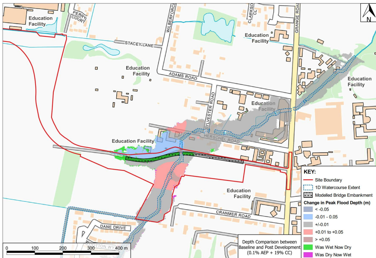
Plate TR13.1-5-3 – Depth Comparison between baseline and proposed model (0.1% AEP + 19%CC)
