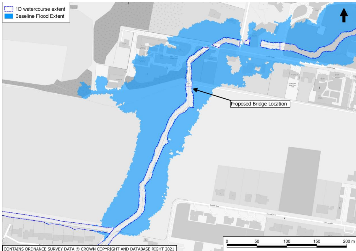
Plate TR13.1-1-2 – Baseline Flood Extent 1% AEP with 19% climate change allowance
